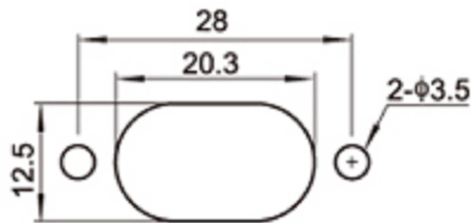
PANEL CUT-OUT
